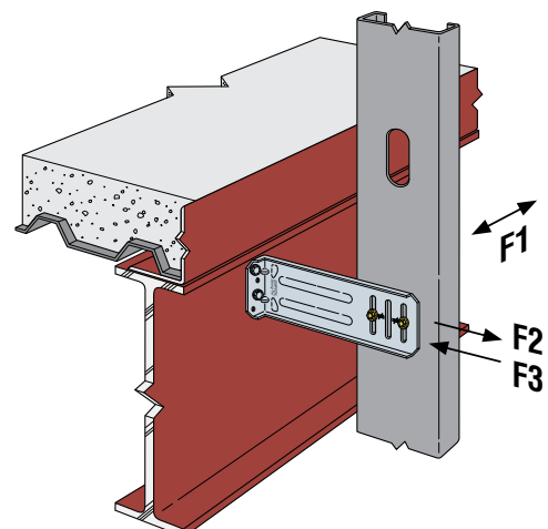
SCB/MSCB Installation at Fascia Beam
