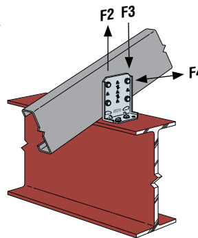
Typical FCB Installation for Roof Rafters
