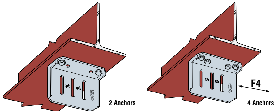
SCW5.5 Anchor Layout
