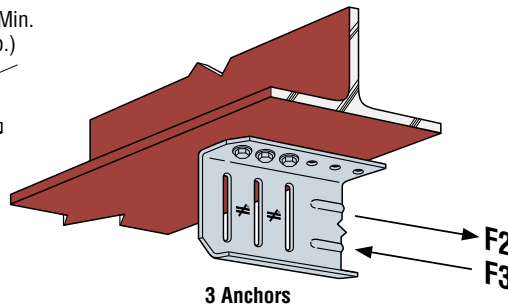
3 Anchors
