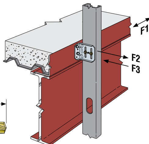
Typical SCB/MSCB Installation
