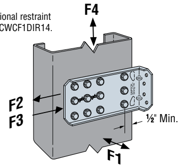
FCB Installation with Max. Fasteners
