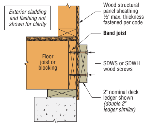
Ledger-to-Band Joist Assembly
